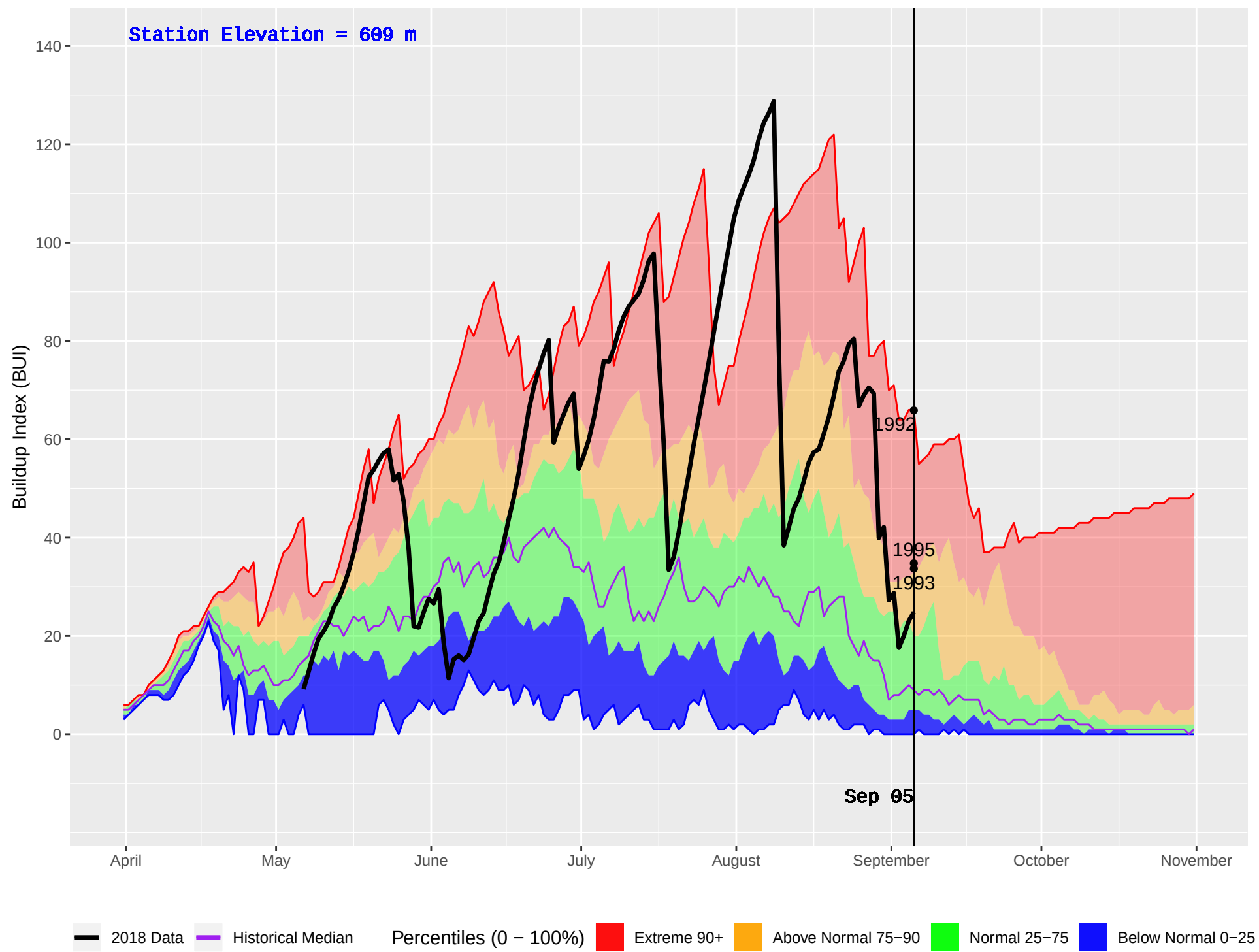
BOB QUINN LAKE (113) : Historical (1984–2016) and Current (2018) Daily Buildup Index (BUI)
